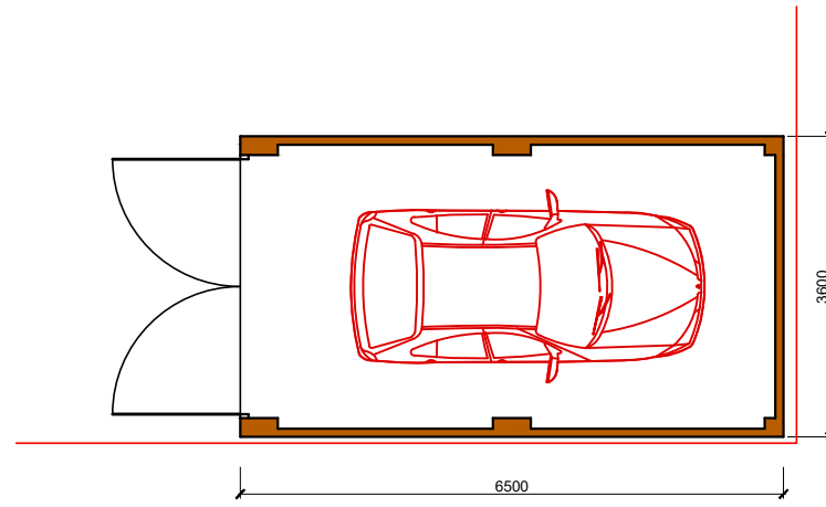
GARAGE FLOOR PLAN 1:100 @ A3
