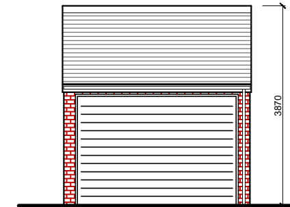
FRONT ELEVATION 1:100 @ A3
