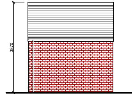
REAR ELEVATION 1:100 @ A3
