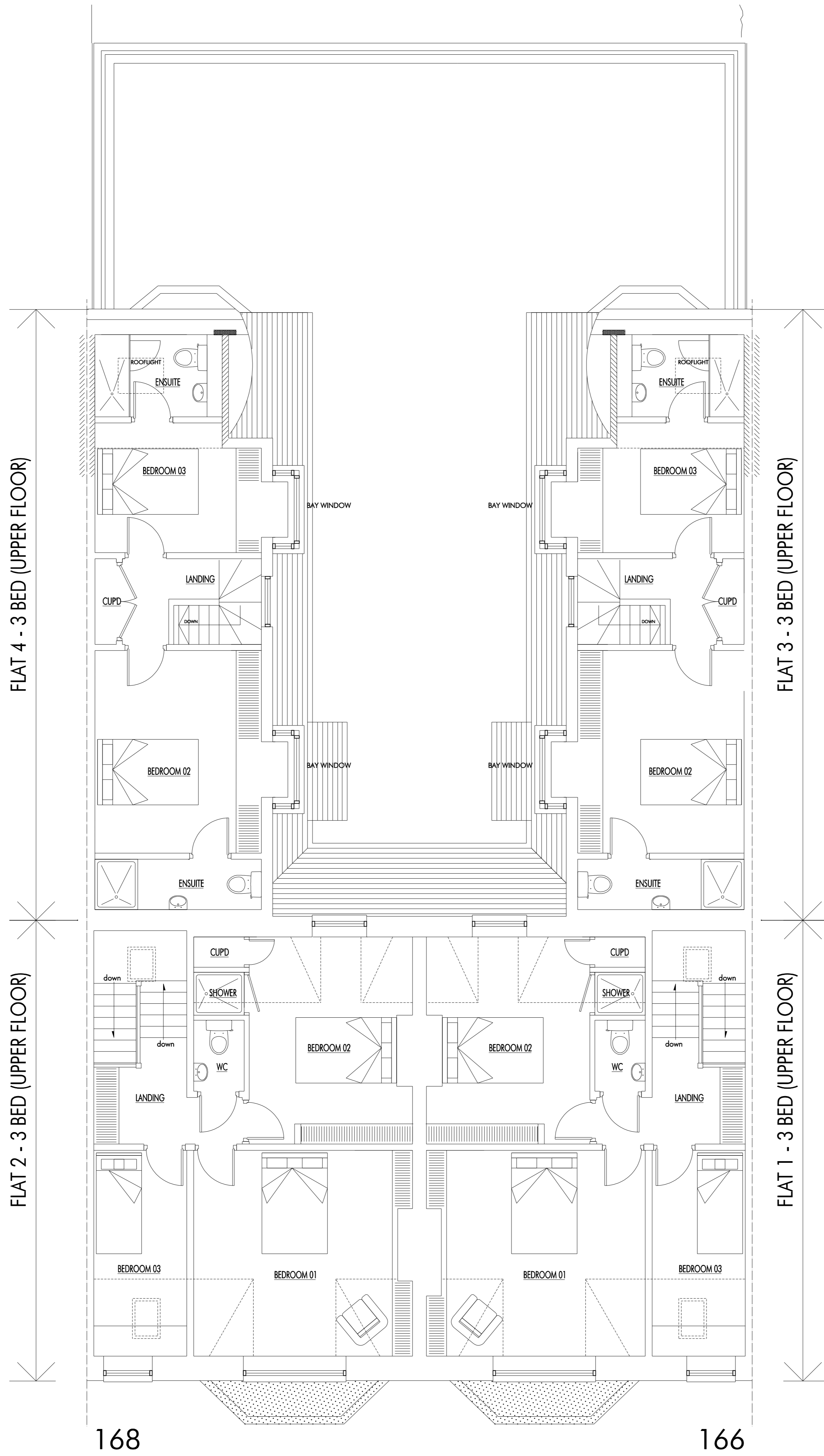
PROPOSED SECOND FLOOR PLAN - 1:50
