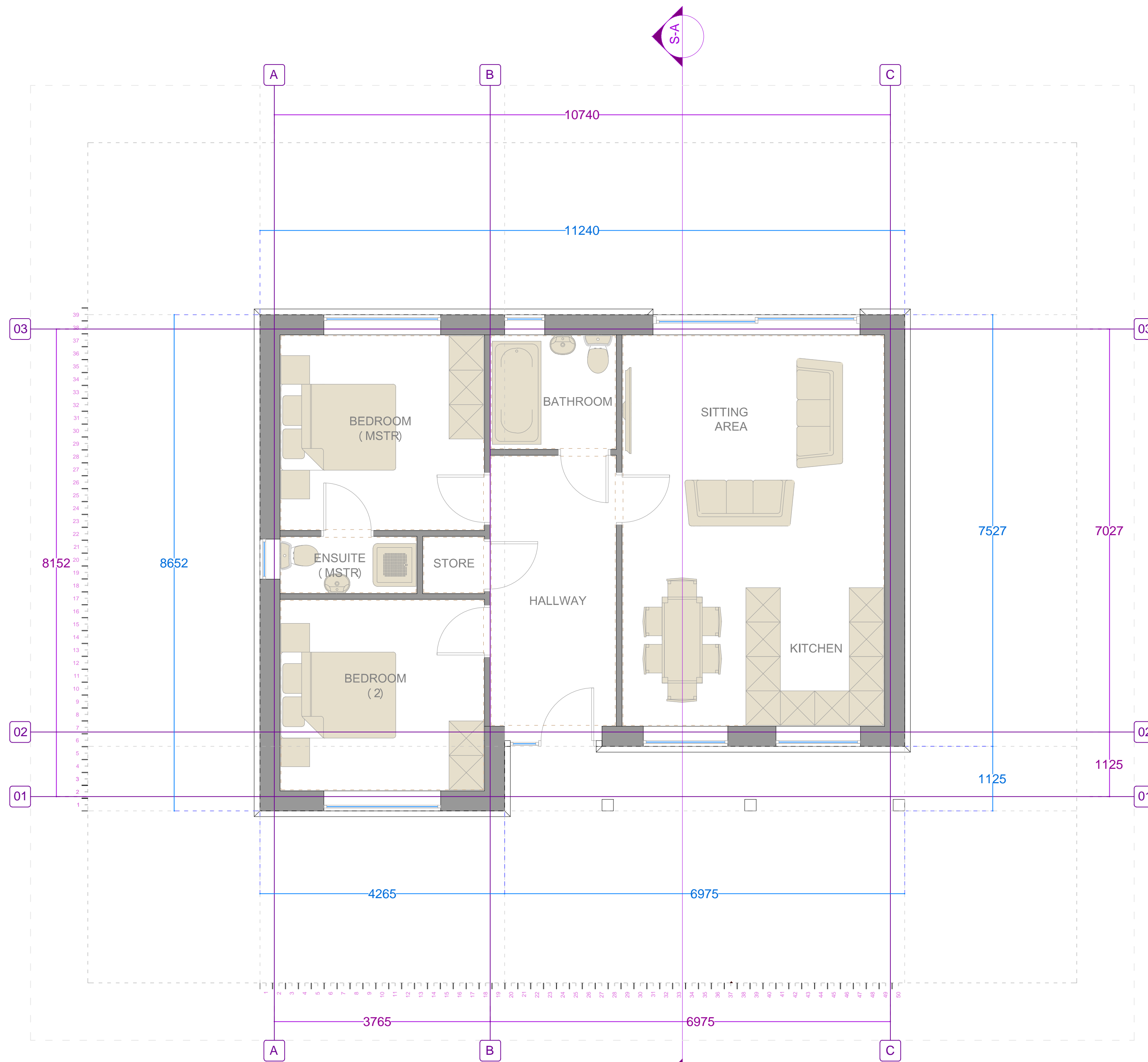
01 Proposed Ground Floor Plan - Type P01 GA Internal Area = 76sqm External Area = 89sqm Scale Bar 0 1 2 3 4 5
