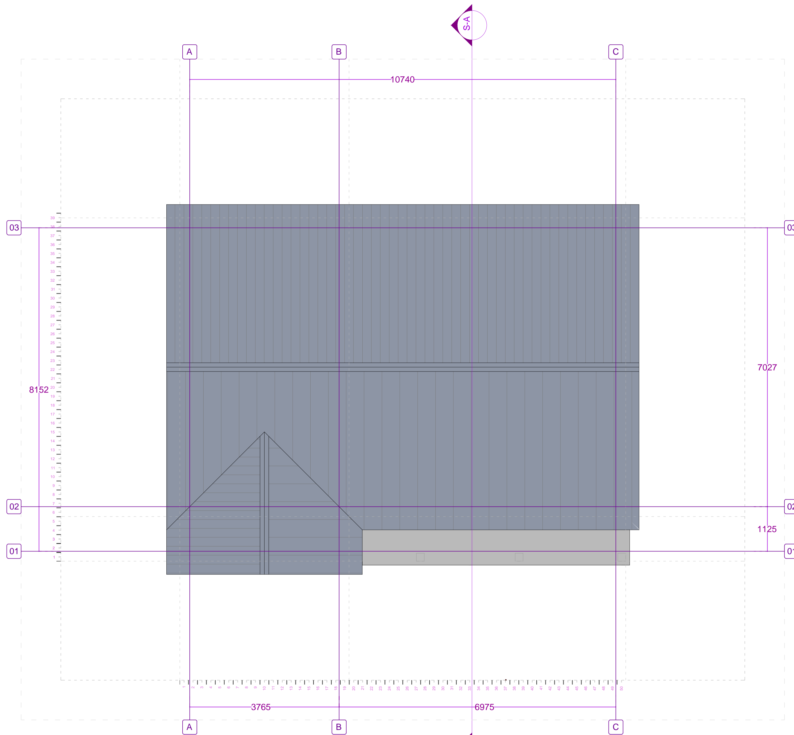
02 Proposed Roof Plan - Type P01 GA
