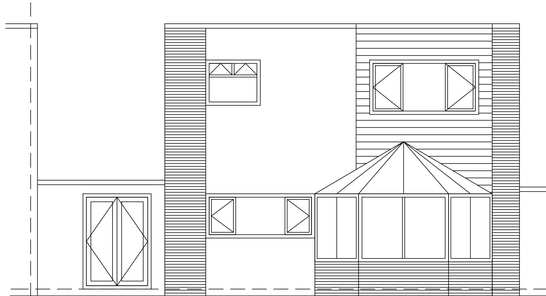
EAST ELEVATION
