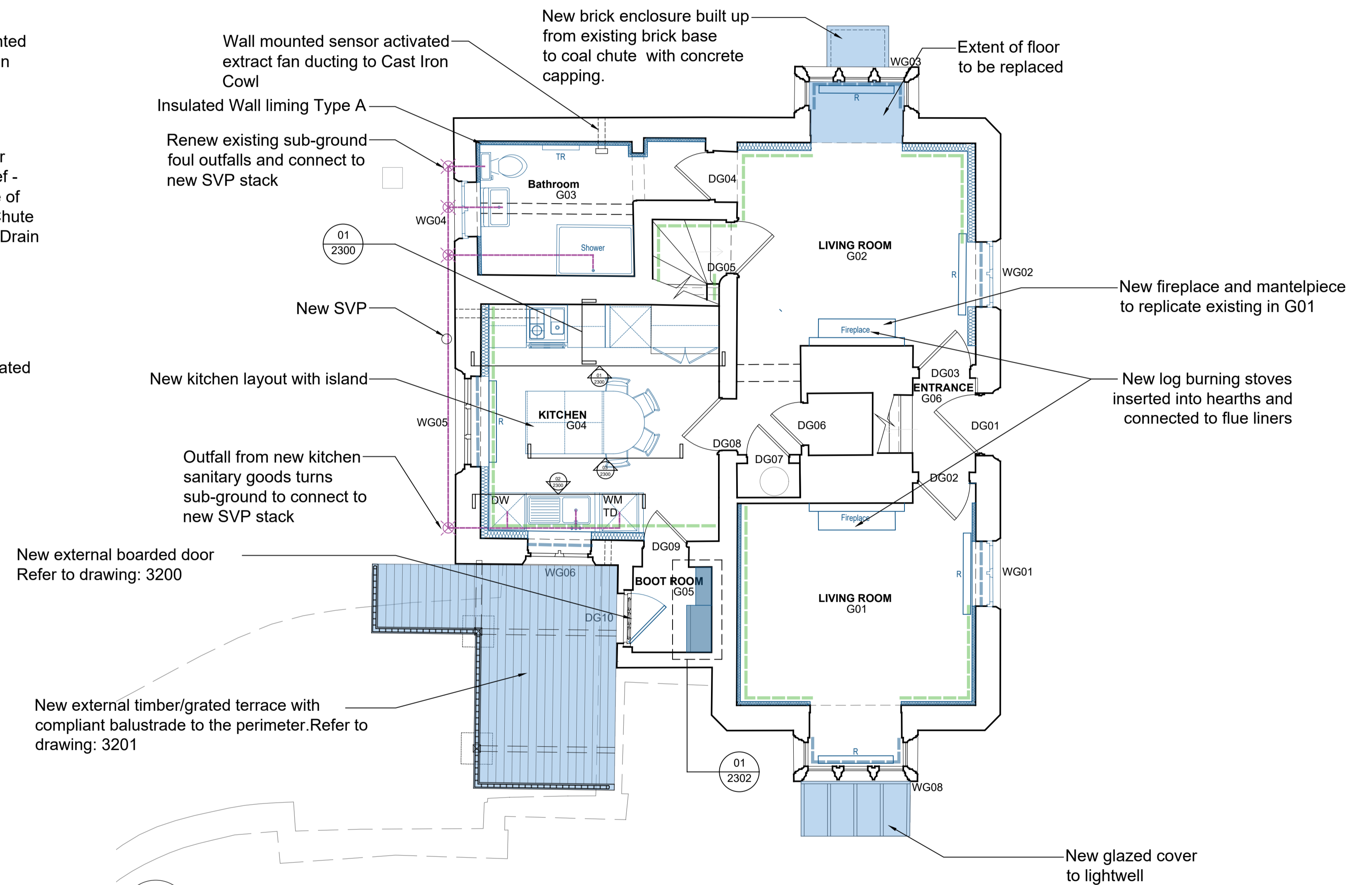
03 Ground Floor 2001 1:50 @ A1
