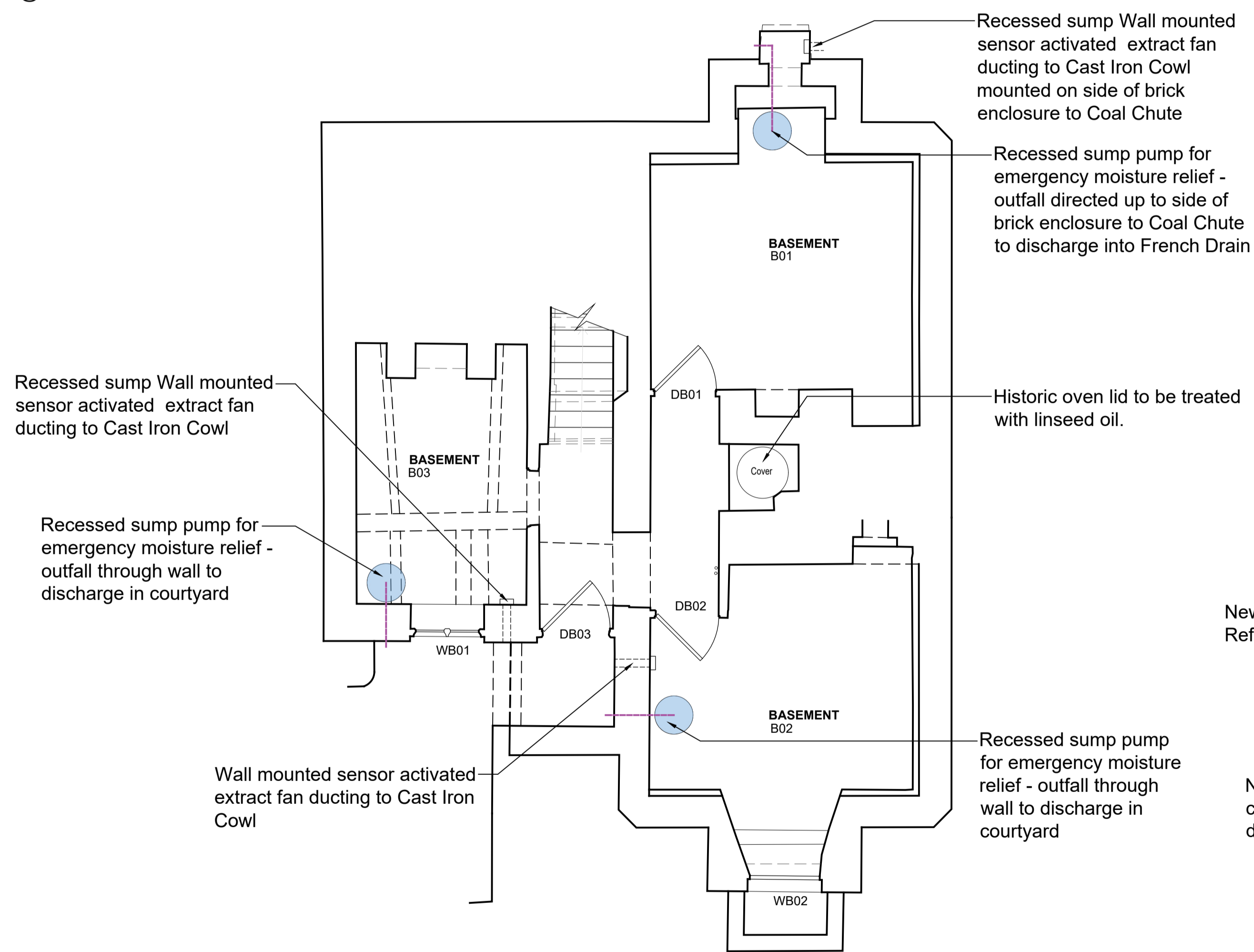
01 Site Plan 2001 1:500 @ A1
