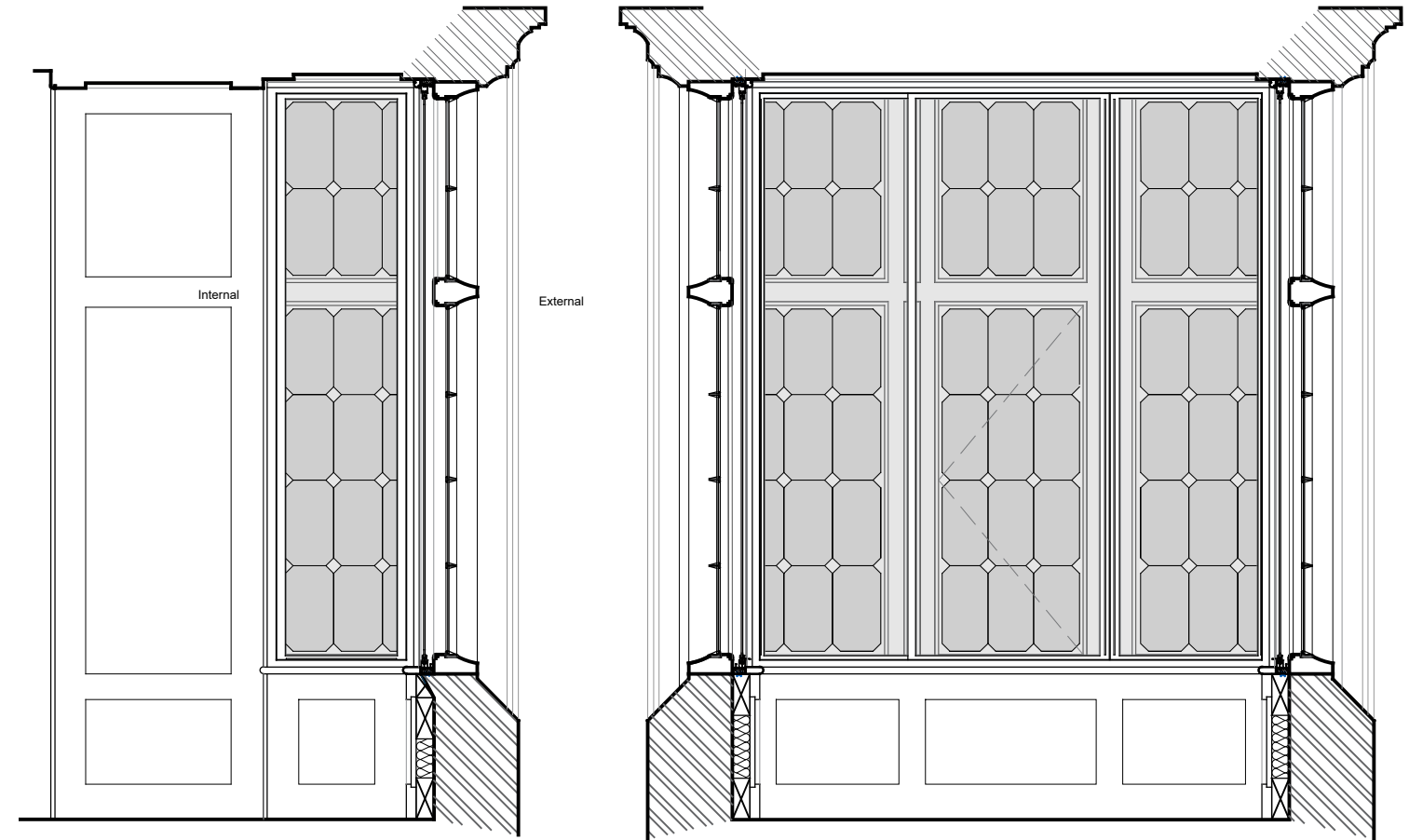
Proposed Secondary Glazing to Existing Window
