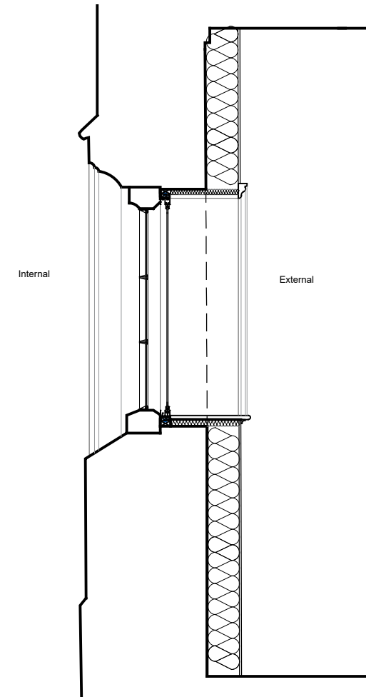
Proposed Secondary Glazing to Existing Window
