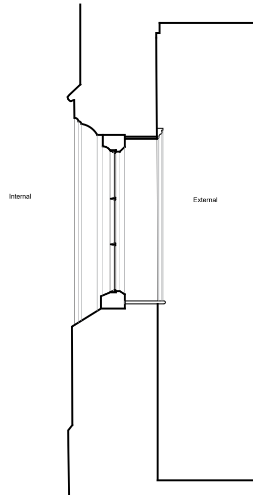
Existing Window
