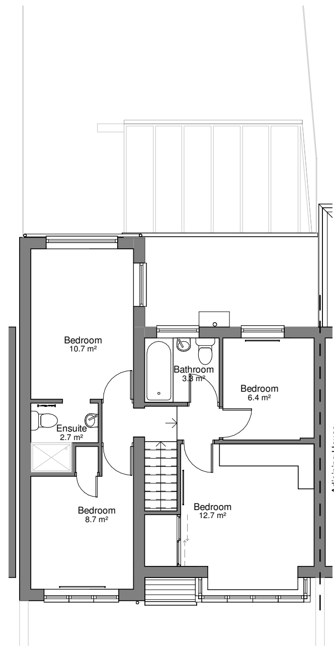
First Floor Plan - Existing 1 : 100
