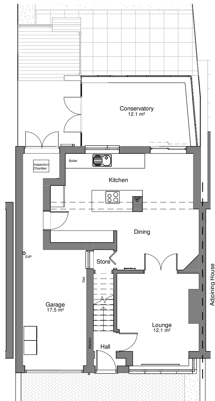
Ground Floor Plan - Existing 1 : 100
