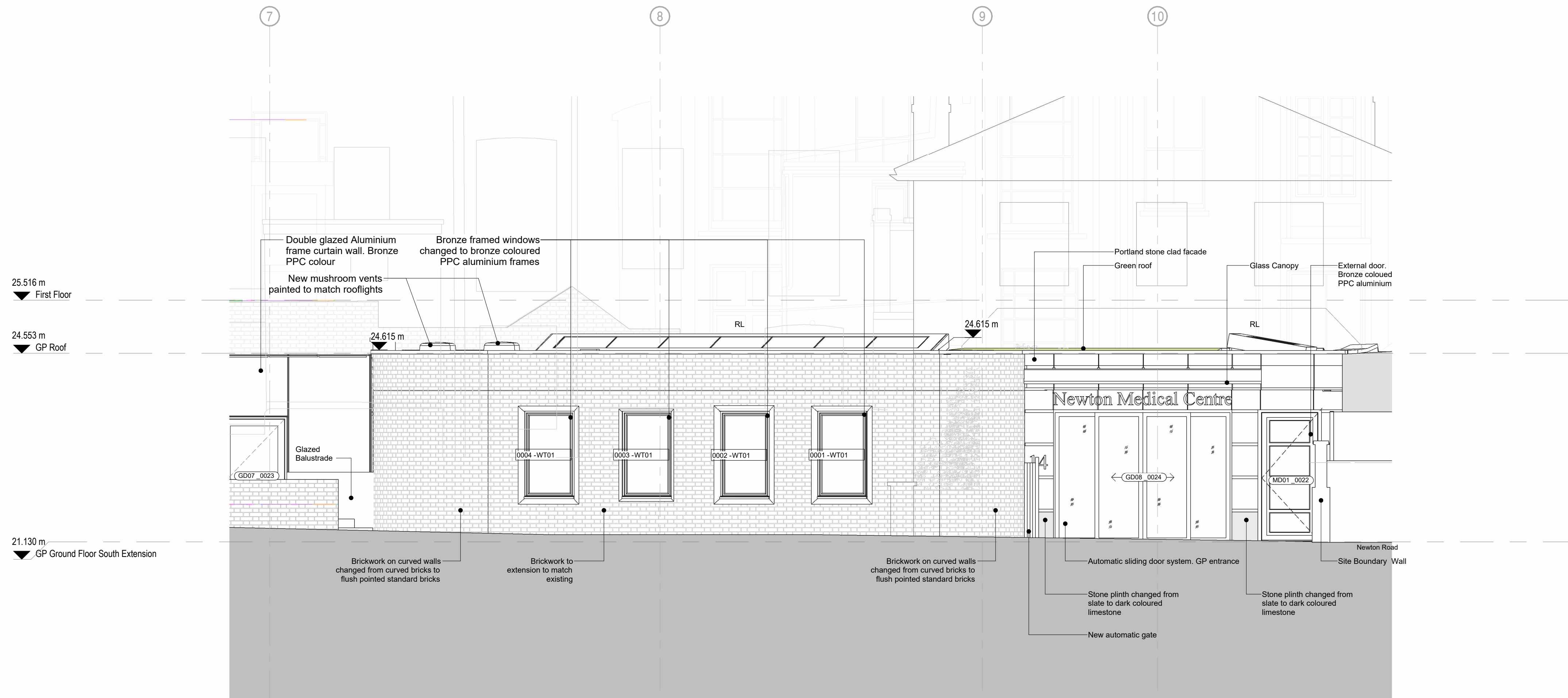
1 West Elevation 1 : 50
