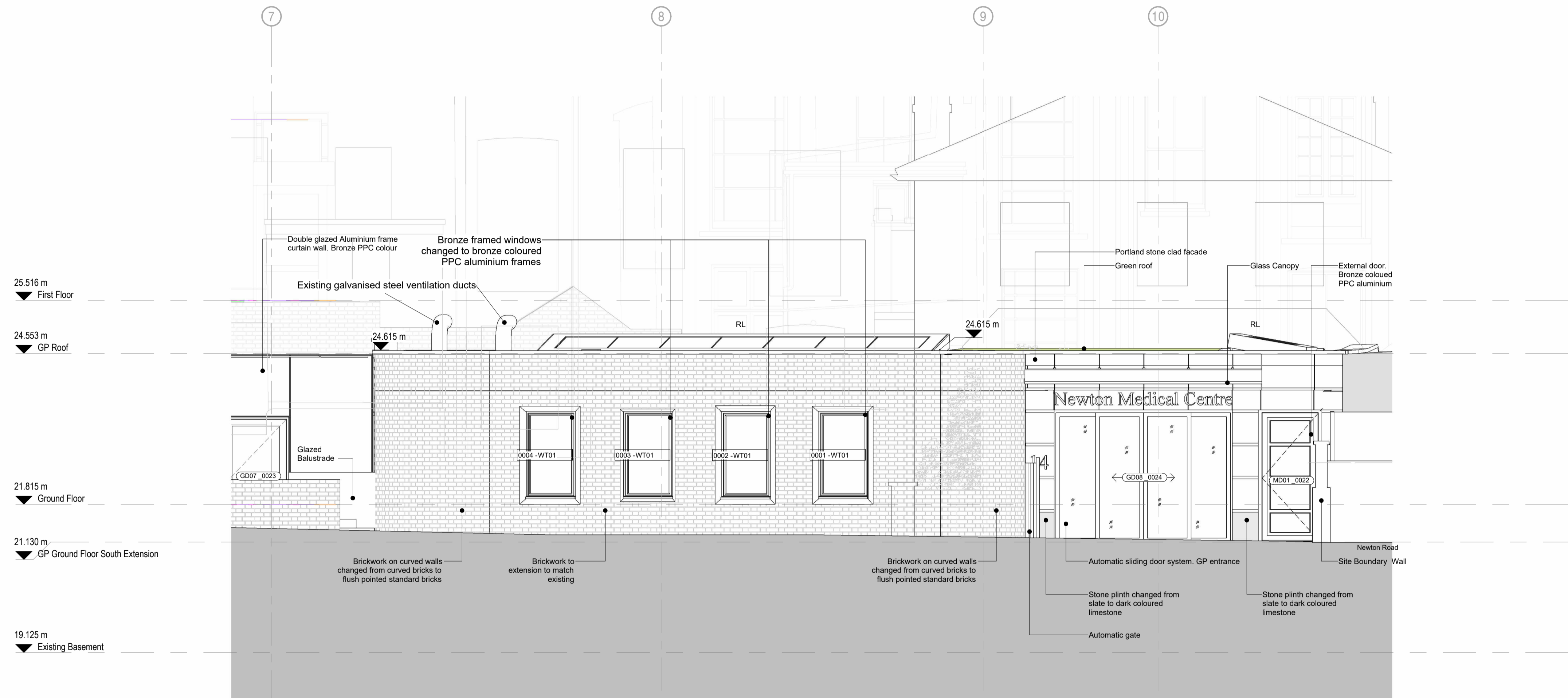
1 West Elevation 1 : 50
