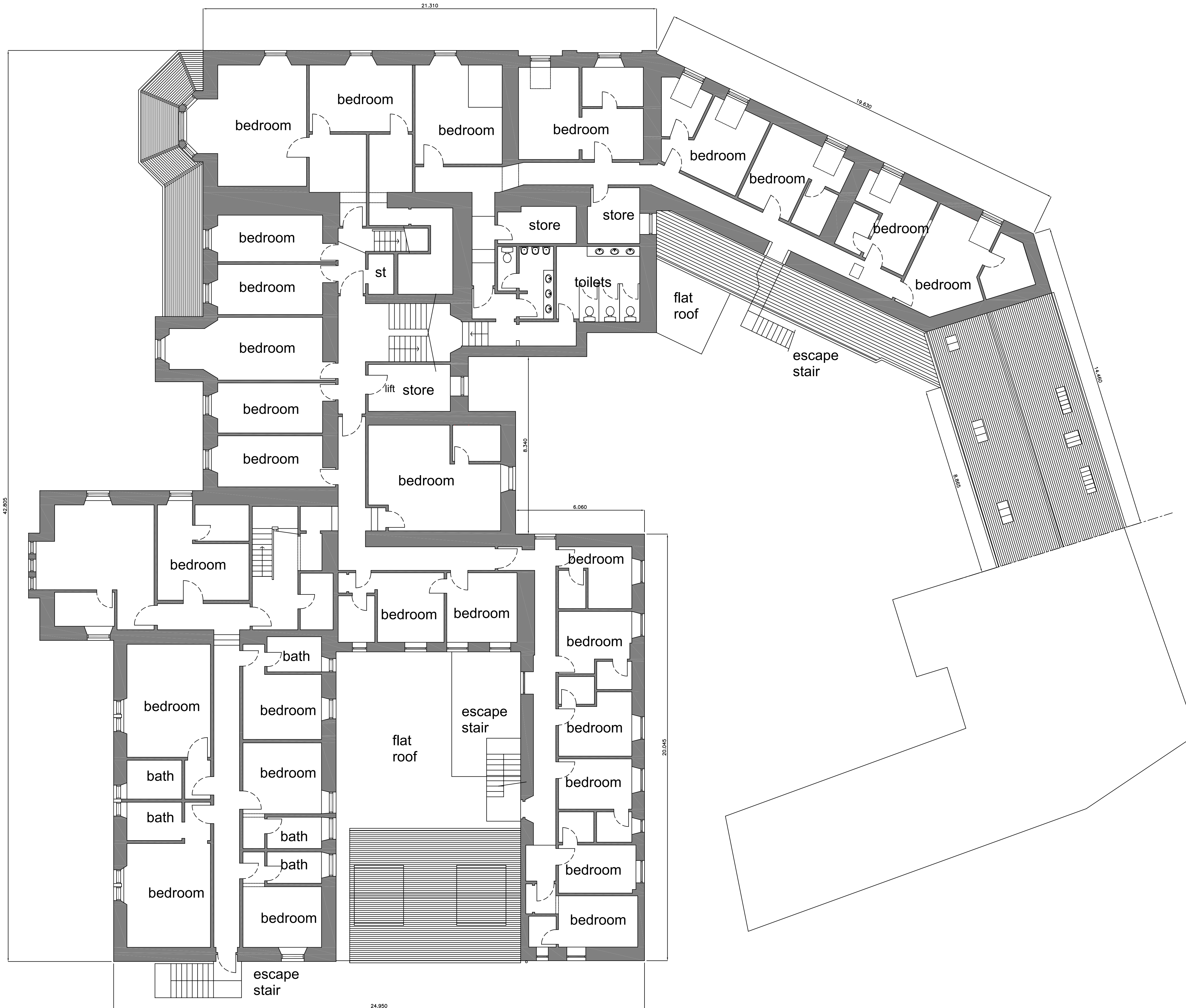
EXISTING FIRST FLOOR PLAN. 1:100.
