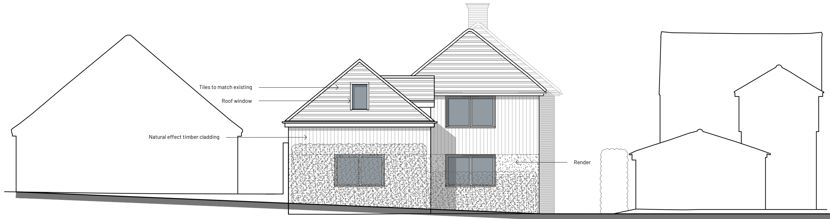
FRONT ELEVATION (STREET SCENE) (NORTH FACING)
