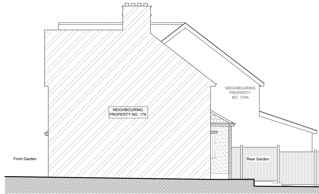
6 Existing North East Elevation 1:100 - Right Flank
